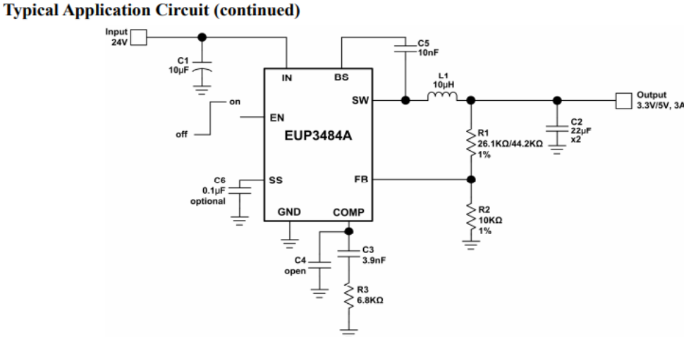
Figure2. 24V to 3.3V/5V Application Circuit
